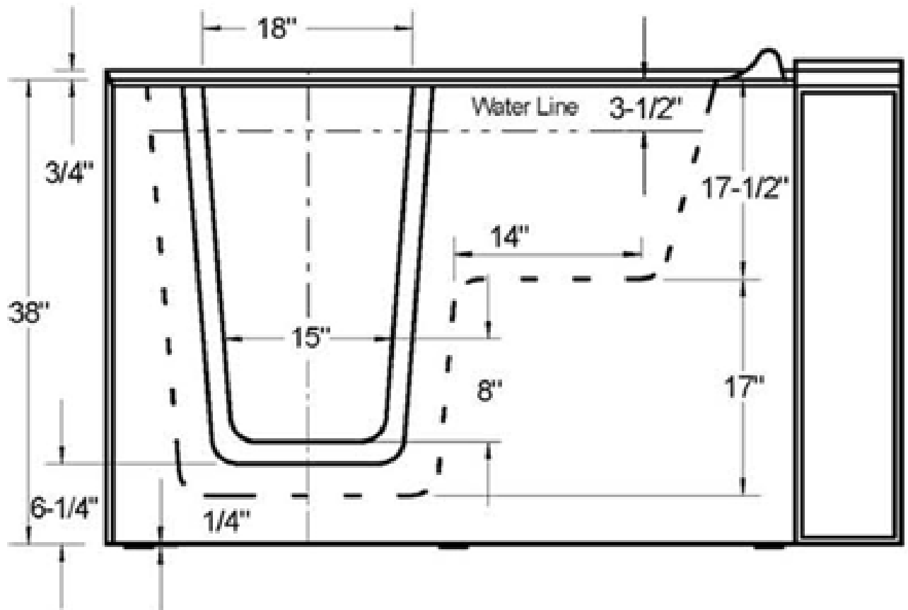
Freedom 30" x 54" x 38"
